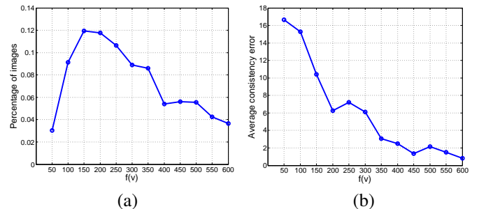
Fig. 10. The impact of VP strength on the accuracy of dominant VP detection. We show (a) the percentage of images and (b) the average consistency error as a function of our strength measure Eq. (10).
