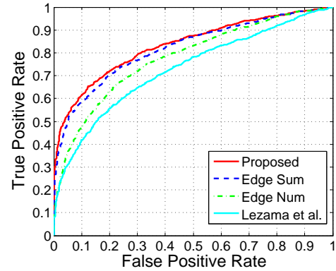
Fig. 9. Experiment results on dominant vanishing point verification.
