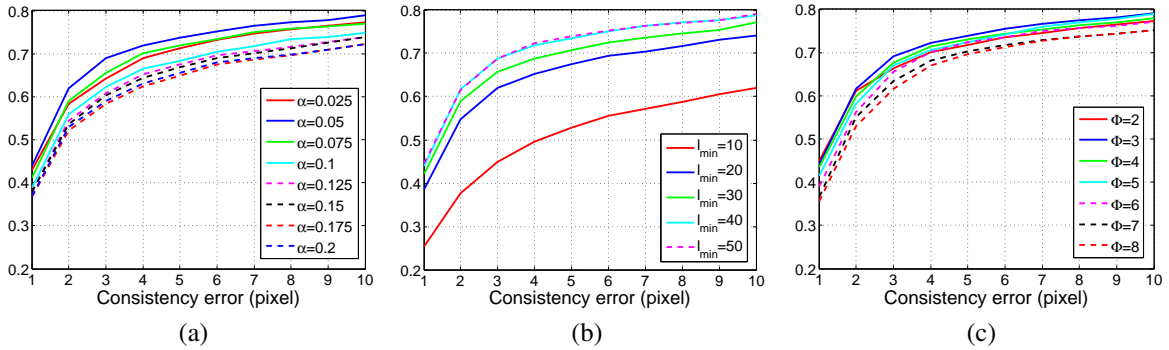
Fig. 6. Accuracy of our method w.r.t. parameters \alpha , l_{\min} , and \phi , respectively.
