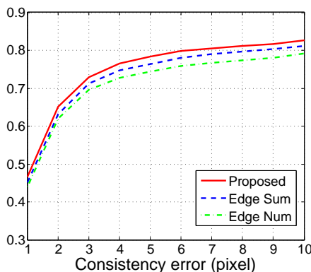
Fig. 8. Experiment results on dominant vanishing point selection.
