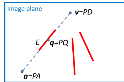
Fig. 7. Illustration of our edge strength measure.
