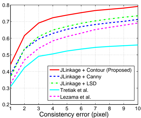
Fig. 4. Vanishing point detection results. We show the cumulative histograms of vanishing point consistency error w.r.t. the ground truth edges (Eq. (6)) for all candidate methods.
