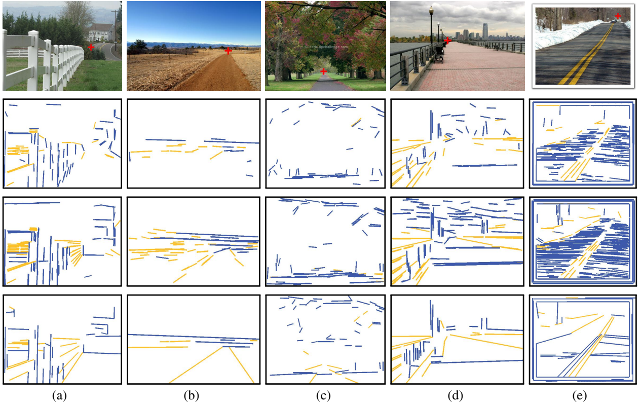
Fig. 5. Comparison of different edge detection methods. The four rows show the original images, and the edges detected by Canny detector, LSD, and our contour-based method, respectively. Yellow edges indicate the edges consistent with the ground truth dominant vanishing point.
