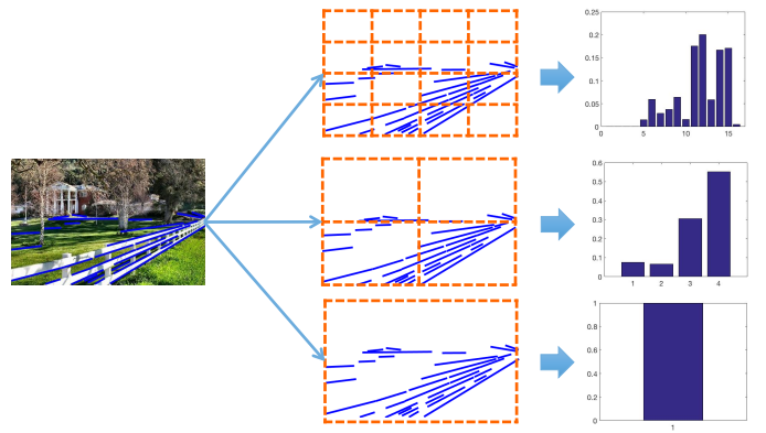
Fig. 11. Illustration of the construction of a three-level spatial pyramid. Given the set of edges \mathcal{E}_i consistent with the dominant VP, we subdivide the image at three different level of resolutions. For each resolution, we count the number of edge points that fall into each bin to build the histograms H_i^l , l = 0, 1, 2 .
