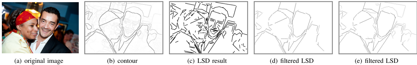
Fig. 3. Filtering the line segments. The parameter \alpha is set to 0.5 and 0.7 in (d) and (e), respectively.
